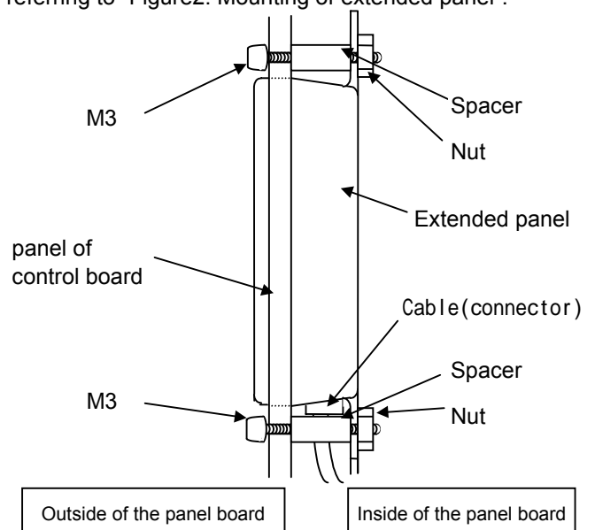
Figure2. Mounting of extended panel
