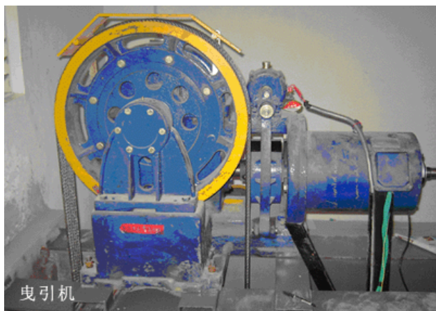
Traction machine
