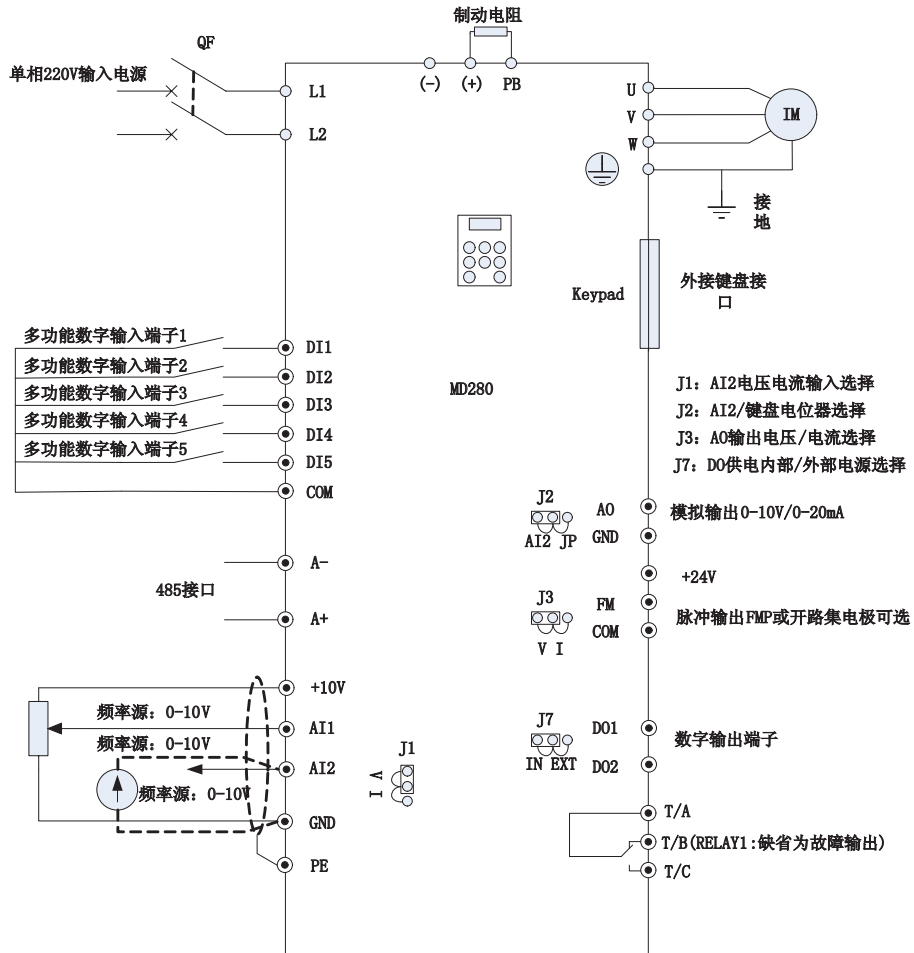
图3-4 MD280S0.4G/MD280S0.7G/MD280S1.5G/MD280S2.2G
