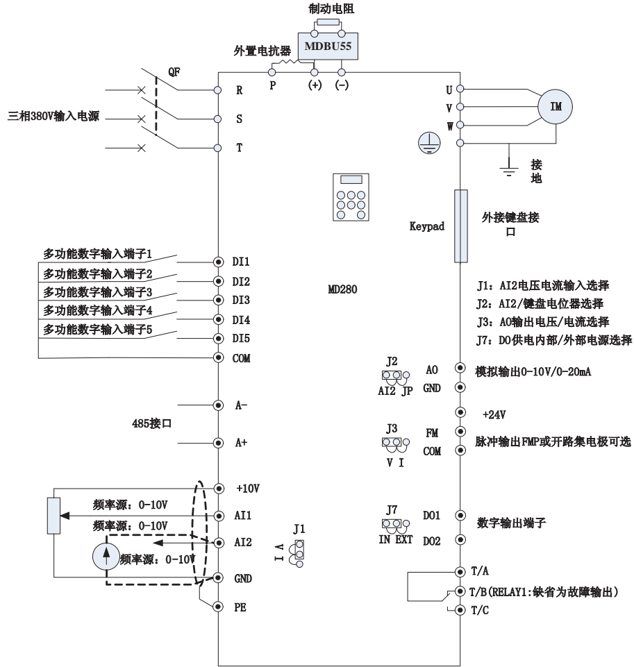
图3-7 MD280T75G/90P~MD280T400G/450P外置电抗器接线示意图
