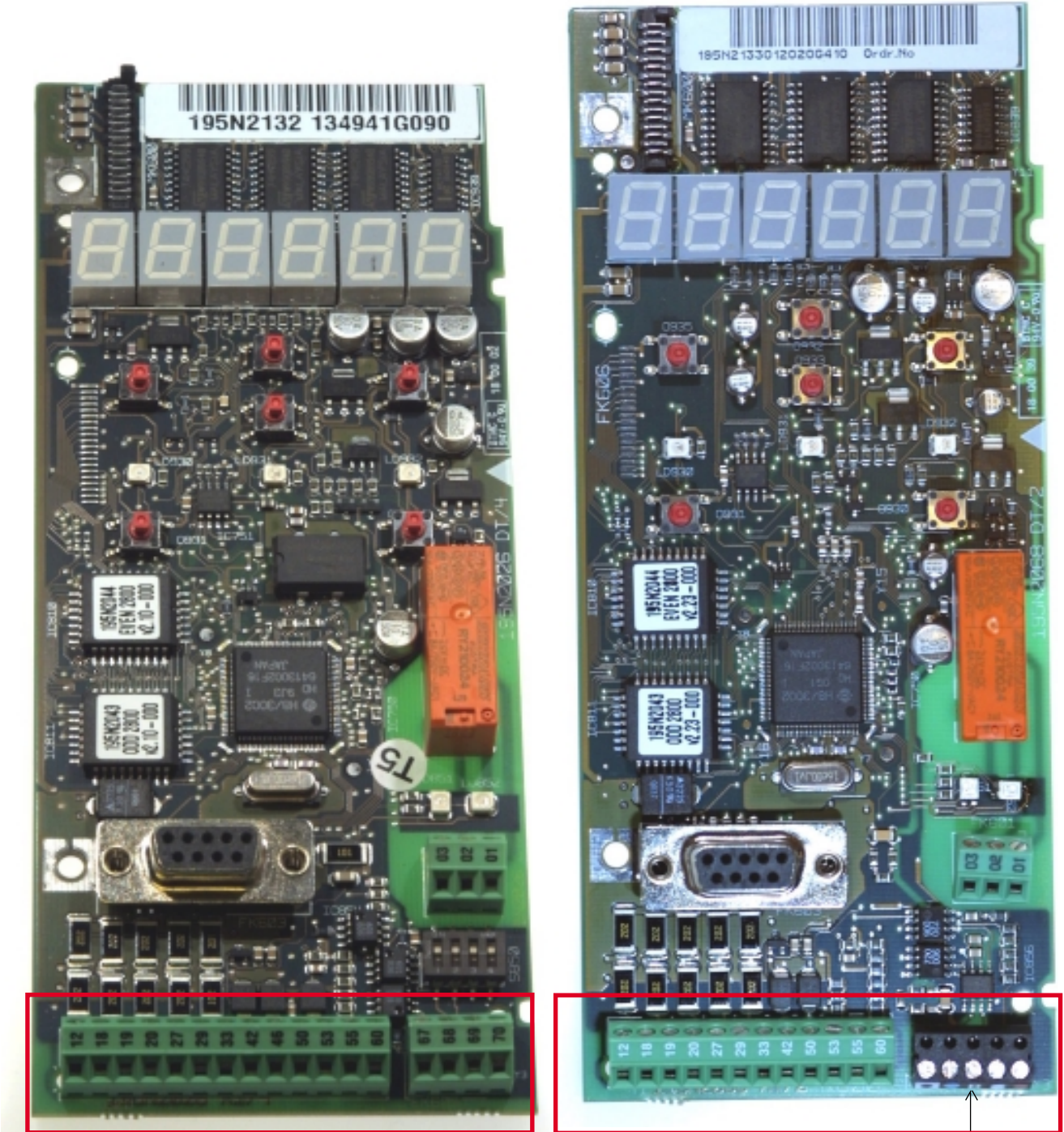
Profibus card
