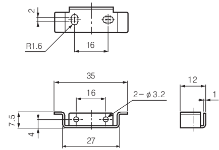
Bracket
