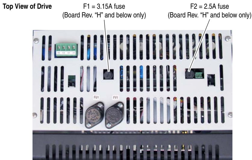
Frame B Switching Power Supply Fuse Location
