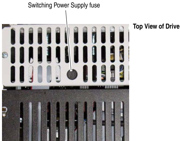
Frame A Switching Power Supply Fuse Location
