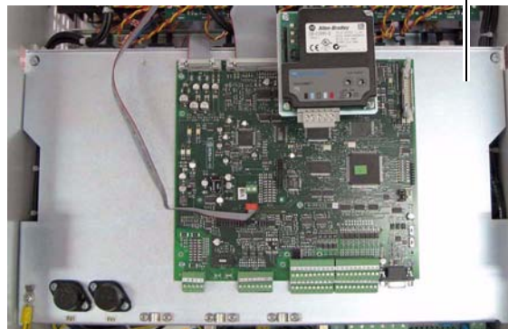
Front of drive shown with top protective cover removed. Control EMI shield
