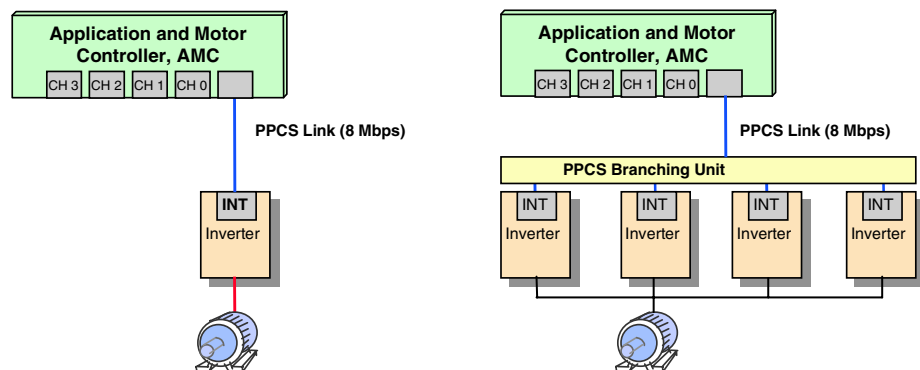
Figure 3-3 Control of single and parallel inverter units
