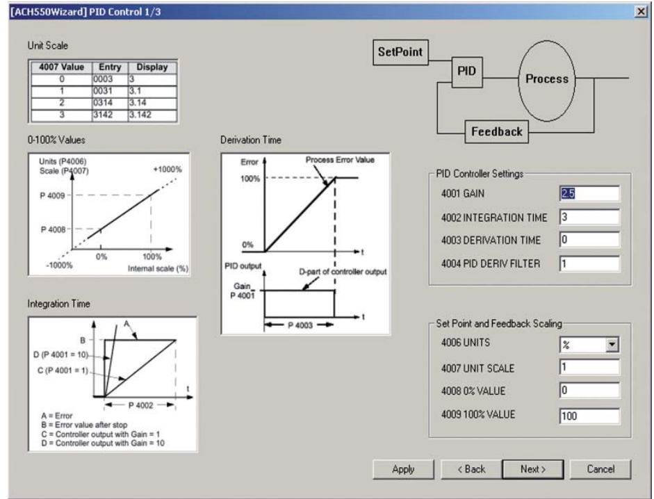
PID control wizard
